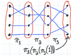
DYNAMIC GRAPHS
