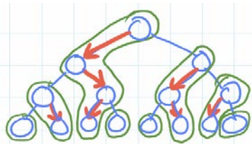
DYNAMIC OPTIMALITY
