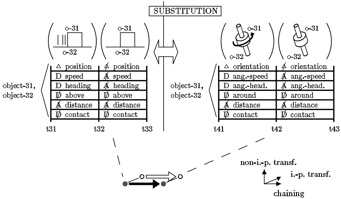
Figure 7: An exploratory information-preserving transformation of type substitution.
